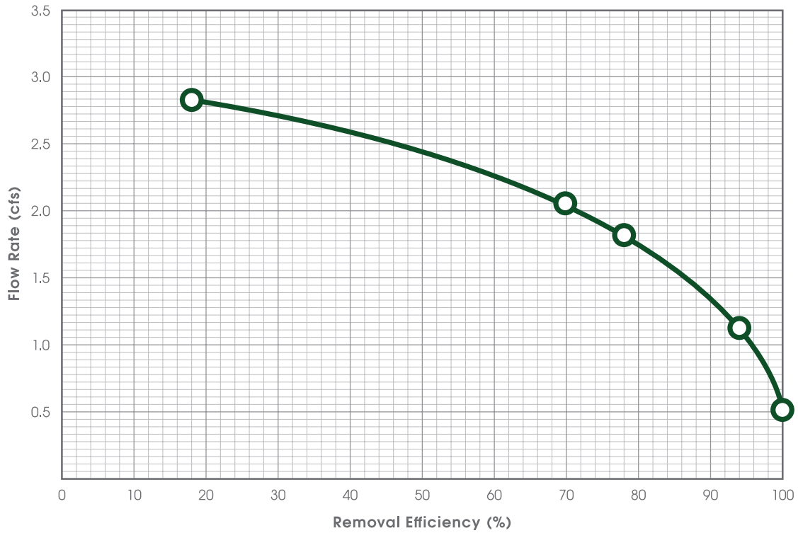
STKS-18, 4'x2' Tank, 1/16" Particles @ 200 mg/L
