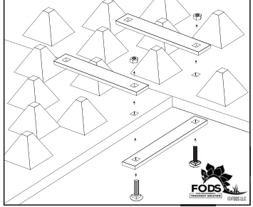
STANDARD T-MAT CONNECTION
