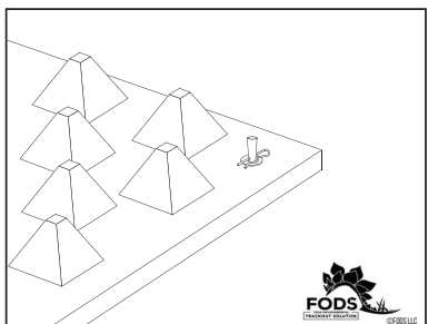
CORNER FORM STAKE ANCHOR SYSTEM
